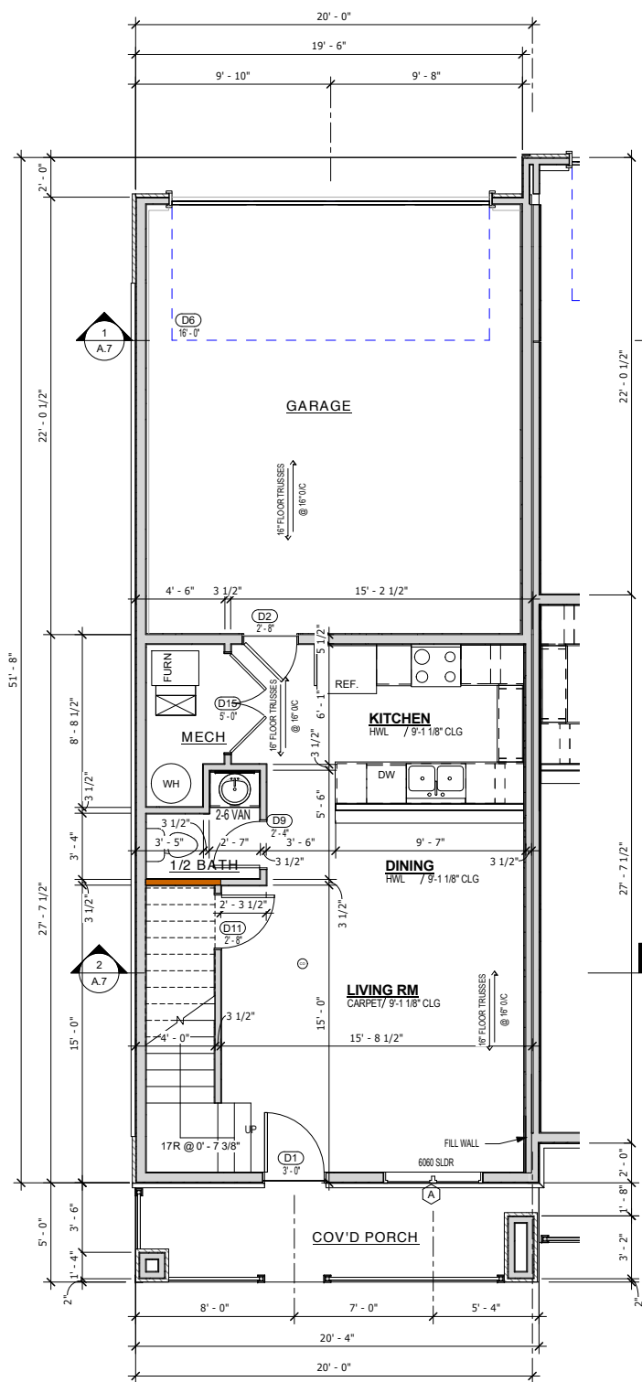
② First Floor - Single Unit Scale: 1/4" = 1'-0"
