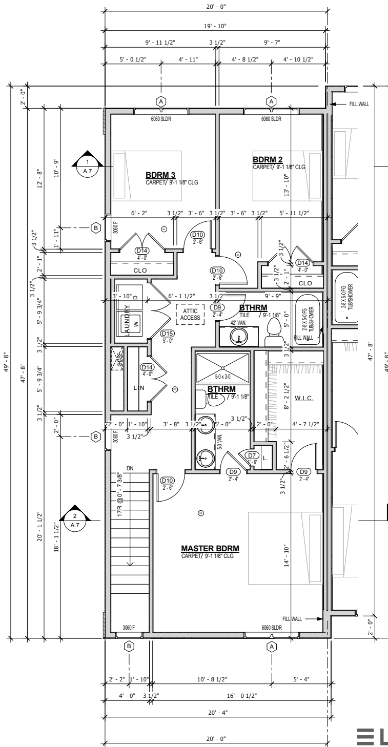
③ Second Floor - Single Unit Scale: 1/4" = 1'-0"
